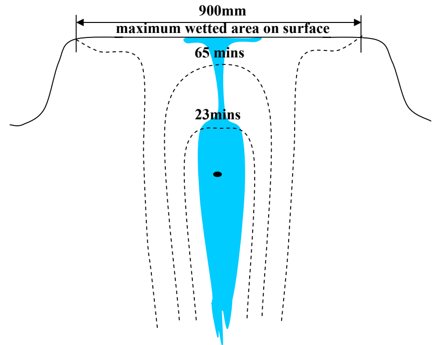
T-tape 8l/hr/lm
